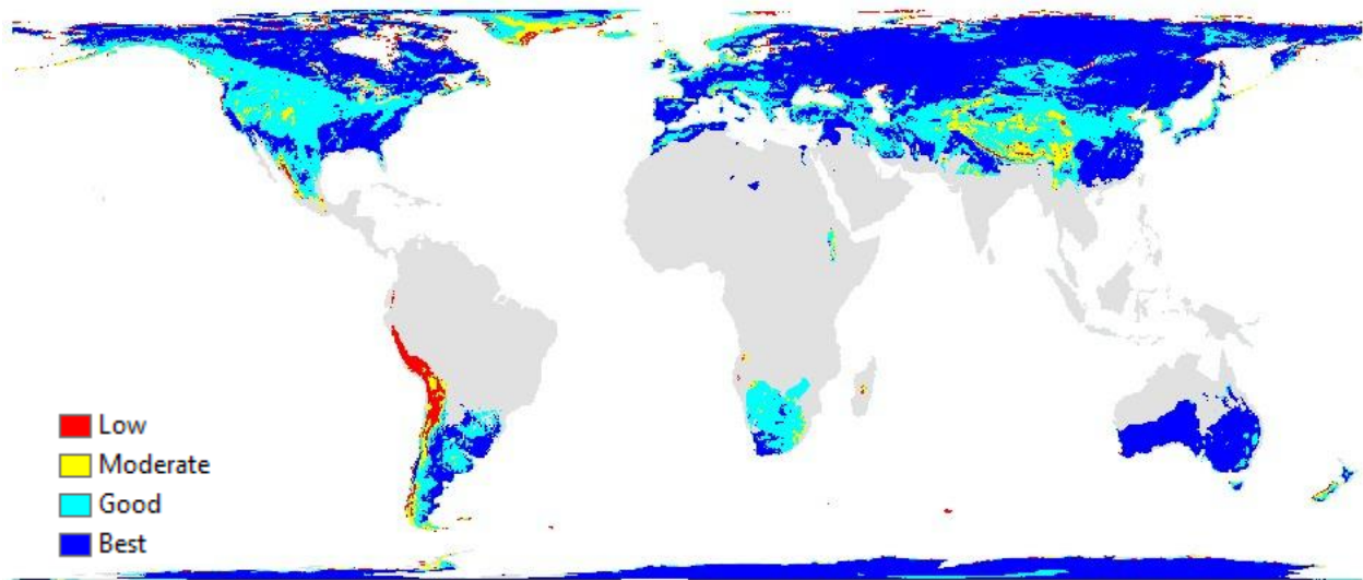
Figure 2: FT-ESDR annual quality assurance (QA) map for selected year of record 2012, aggregated into low (estimated mean annual spatial classification agreement < 70%), moderate (70-80%), good (80-90%) and best (>90%) relative quality categories. Land areas outside of the FT-ESDR domain are denoted by grey shading.
