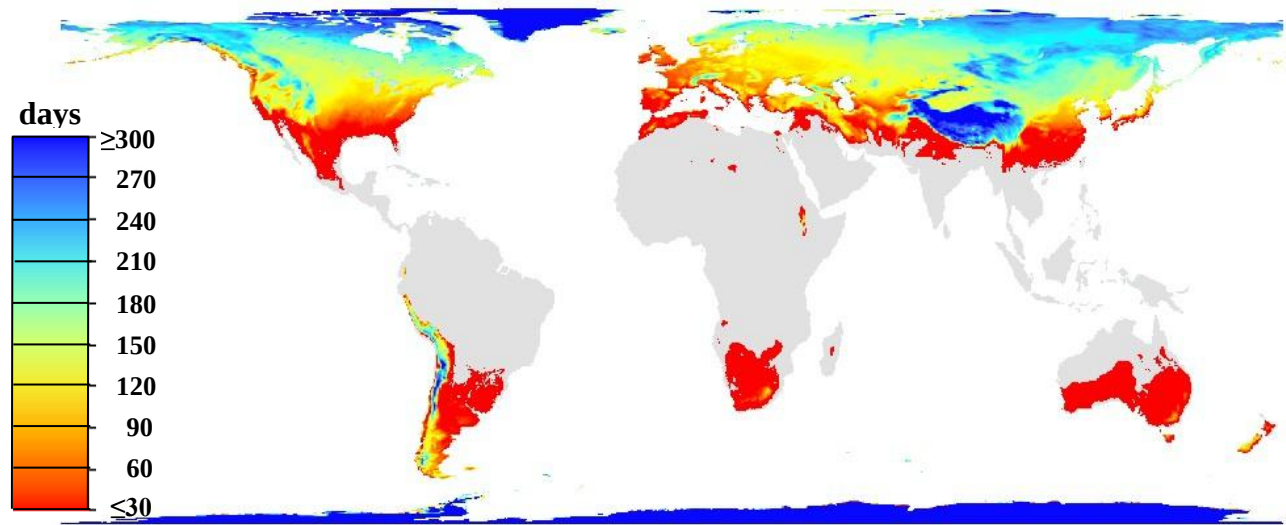
Figure 1: Mean annual frozen season (frozen or transitional status; 1979-2020) over the global FT-ESDR domain; white and grey colors denote respective open water bodies and land areas outside of the FT-ESDR domain.
