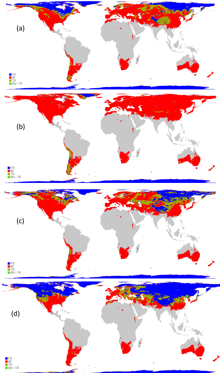
Figure 3: Daily combined (CO) FT-ESDR classification results for selected year of record 2016, where: (a) DOY (Day of Year) =100, (b) DOY=200, (c) DOY=300, and (d) DOY=360; white
