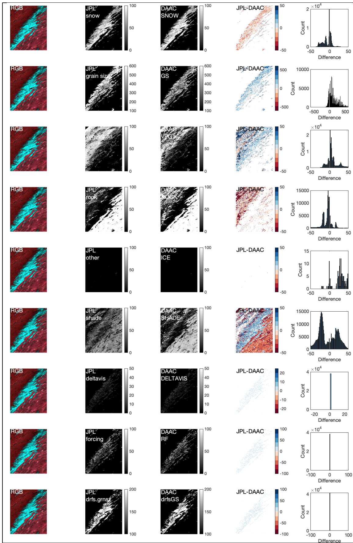
Figure 2: Differences in JPL MODSCAG and MODDRFS and NSIDC DAAC MODSCGDRF layers in early spring April 9, 2023. See Figure 1 for complete description.
