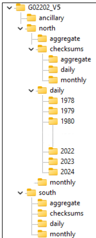
Figure 1. Directory Structure
