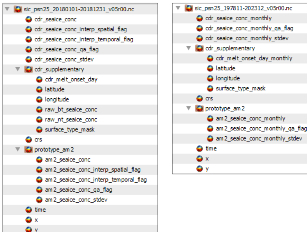
Figure 2. File Contents of a Northern Hemisphere daily aggregated NetCDF file (left) and Northern Hemisphere monthly aggregated NetCDF file (right).
